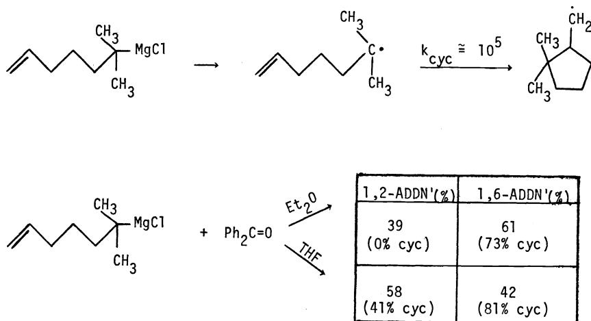
Fig. 18. 1,1-Dimethyl-5-hexenylmagnesium chloride as a free radical probe.
