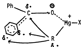
Fig. 19. Transition state depicting alkyl group transfer
