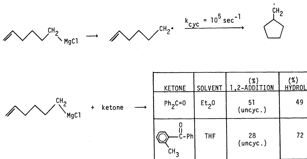
Fig. 17. 5-Hexenylmagnesium chloride as a free radical probe
