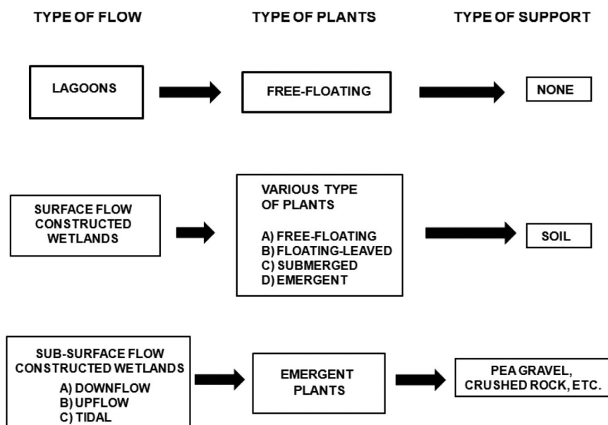
Fig. 1 Classification of phytofiltration systems for wastewater treatment using aquatic plants.
